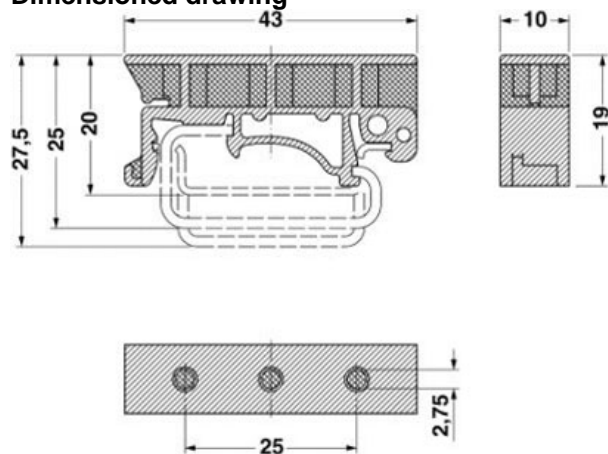
Dimensioned drawing
