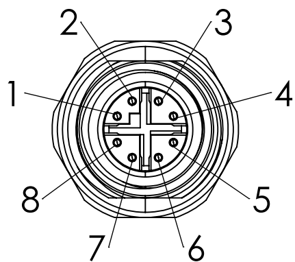
Connector Pinout (Female)
