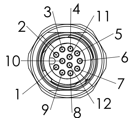
Connector Pinout (Female)
