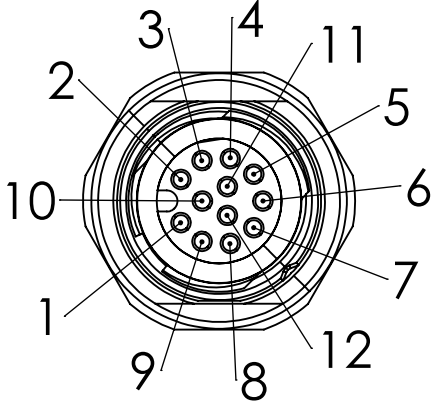
Connector Pinout (Female)
