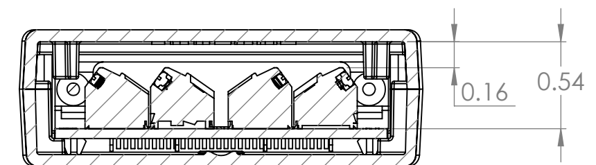
SECTION B-B
