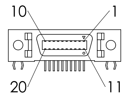
Connector Pinout (Female)
