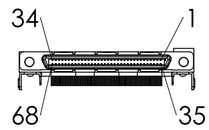
Connector Pinout (Both Female)
