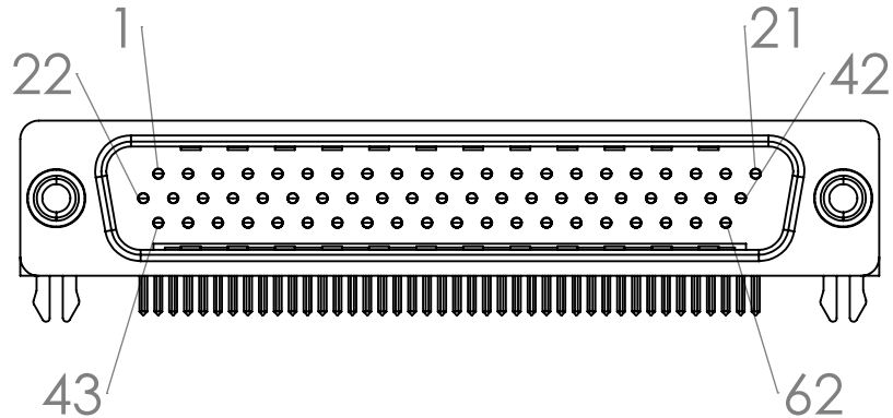
Connector Pinout (Male)
