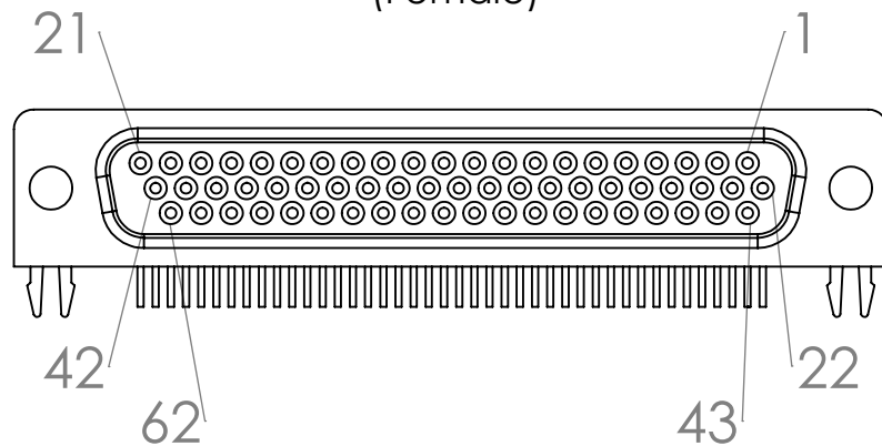
Connector Pinout (Female)
