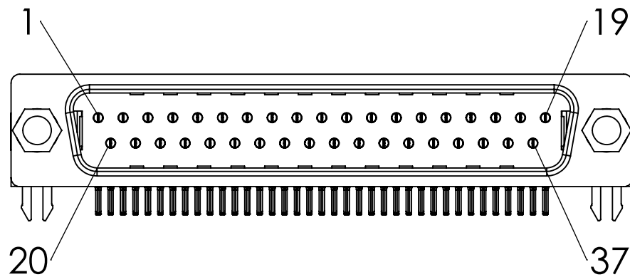
Connector Pinout (Male)
