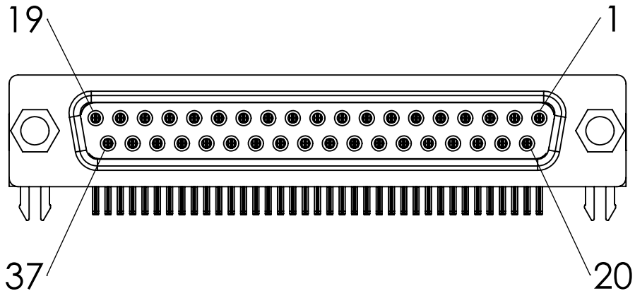
Connector Pinout (Female)
