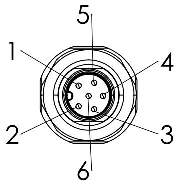
Connector Pinout (Male)
