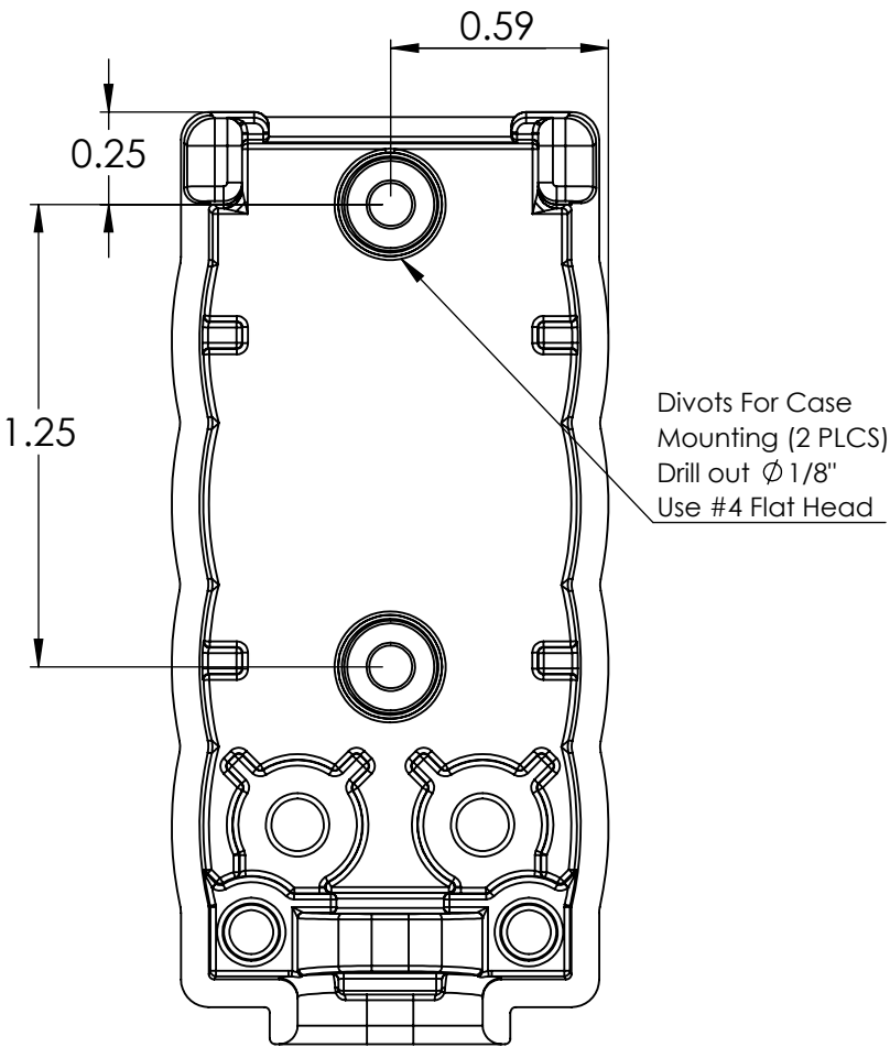
Base, Without Board Installed
