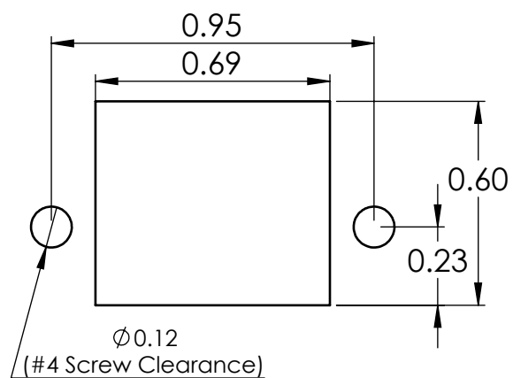
Panel Cutout
