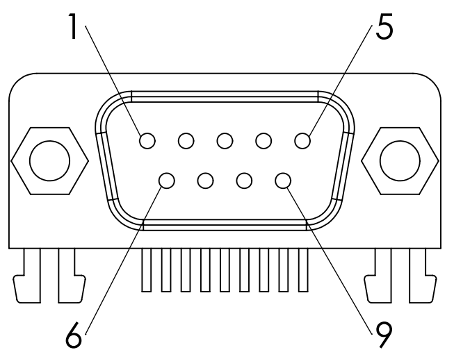
Connector Pinout (Male)
