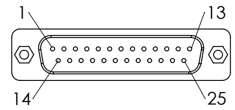
Male Connector
